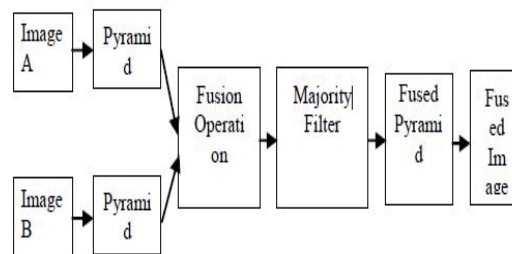
Fig. 4 Laplacian pyramid fusion algorithm
