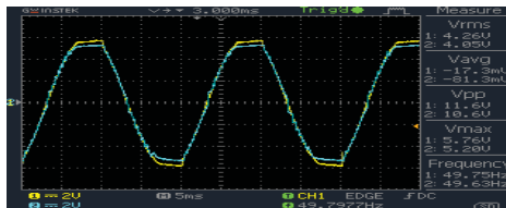
Fig. 16 Waveforms for Grid voltage and inverter voltage at overload condition with resistive load
