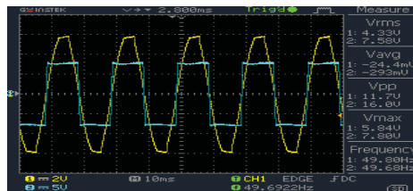
Fig.12 Waveforms of grid voltage and zero crossing detector
