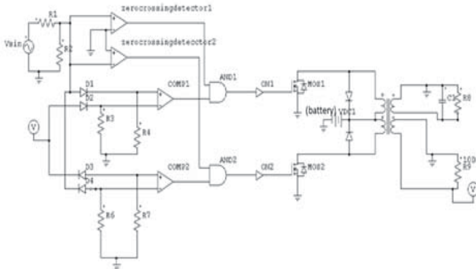
Fig.4 Circuit diagram for grid tracking inverter.
