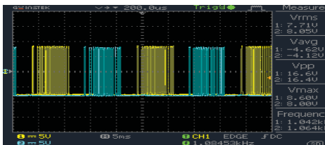
Fig.14 Switching pulses of MOSFETs
