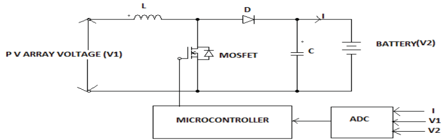
Fig.3 Closed loop boost converter
