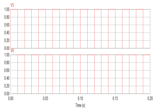
Fig.8 Output voltage from zero crossing detector 1 and zero crossing detector 2
