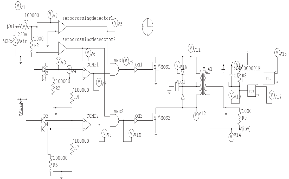
Fig.5 Simulation circuit diagram for grid tracking inverter in PSIM
