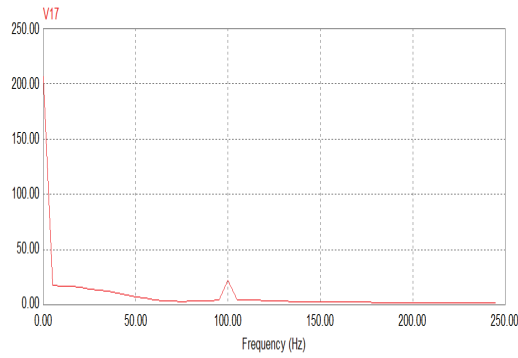
Fig.10 THD analysis
