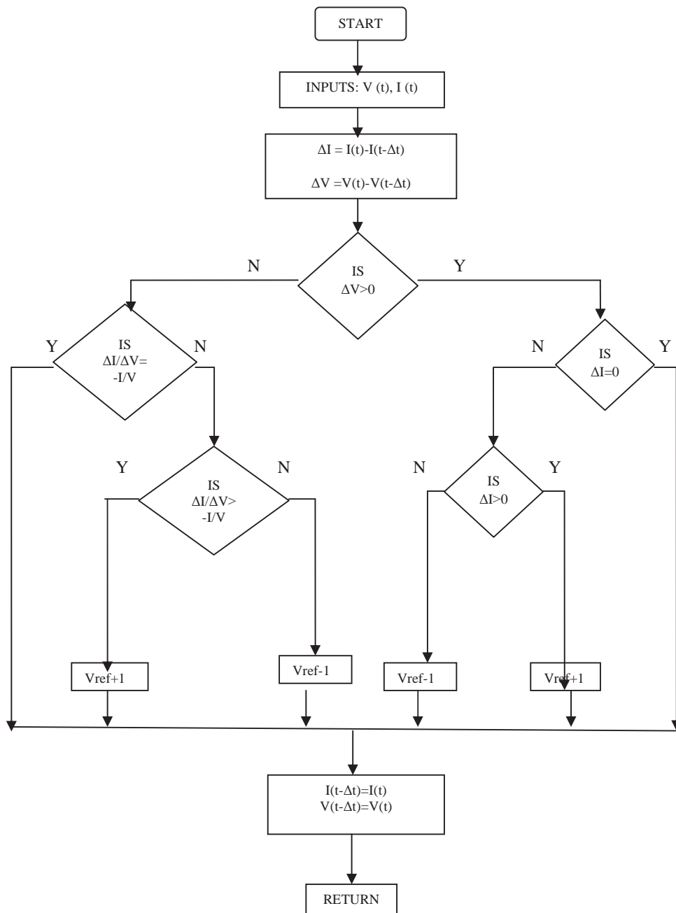
Fig.2 Flowchart for incremental conductance method.
