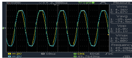
Fig.15 Waveforms for grid voltage and inverter voltage for inductive load
