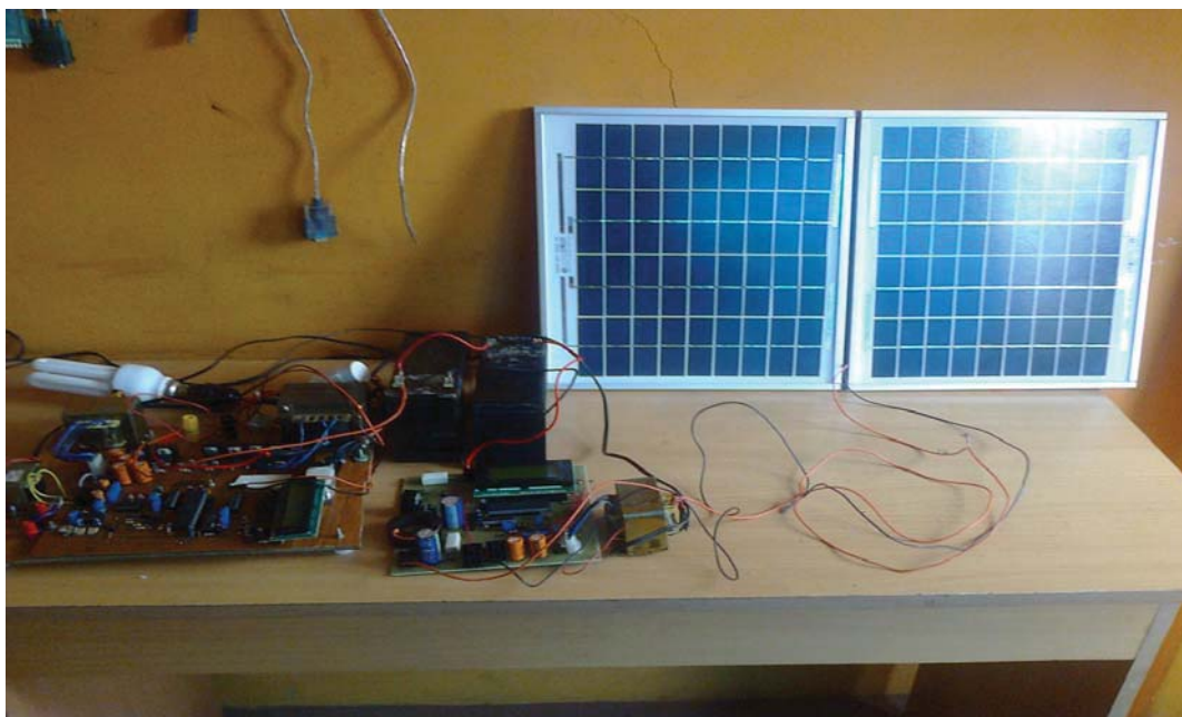
Fig.18 Hardware for the proposed system
