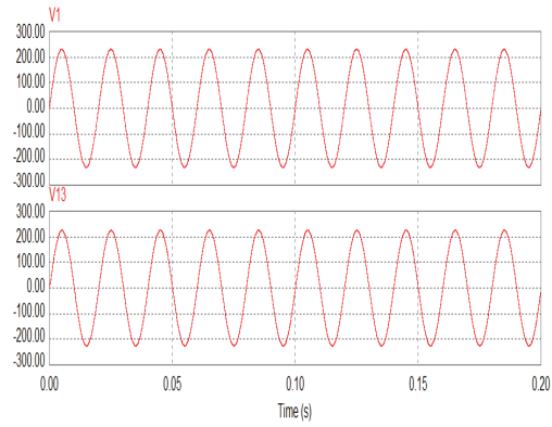
Fig.7 Grid voltage and inverter voltage 230V, 50Hz
