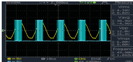
Fig.13 Waveforms of grid voltage and switching pulses of MOSFET 1
