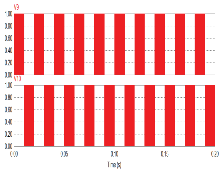
Fig.9 Switching pulses for MOSFET 1 and MOSFET 2
