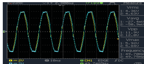
Fig.17 Waveforms for grid voltage and inverter voltage for capacitive load
