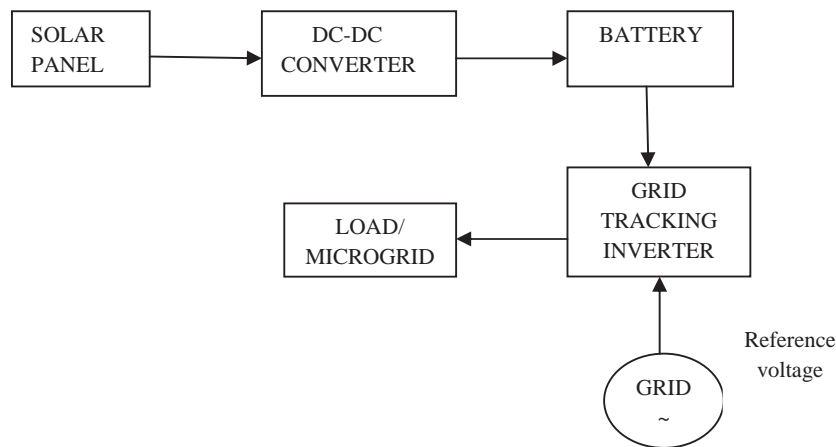
Fig.1 Basic block diagram of grid synchronization
