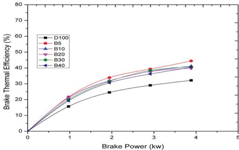
Figure-2 Variation of Brake power with Brake Thermal Efficiency using TSOME Blends.
