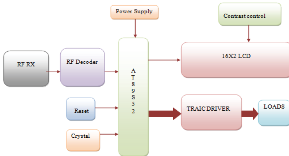
Figure 3: Receiver system
