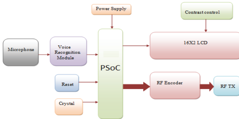
Figure 3: Transmitter system
