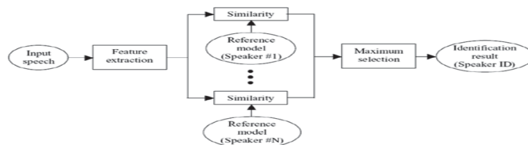
Figure 1: Speaker Identification (Training)
