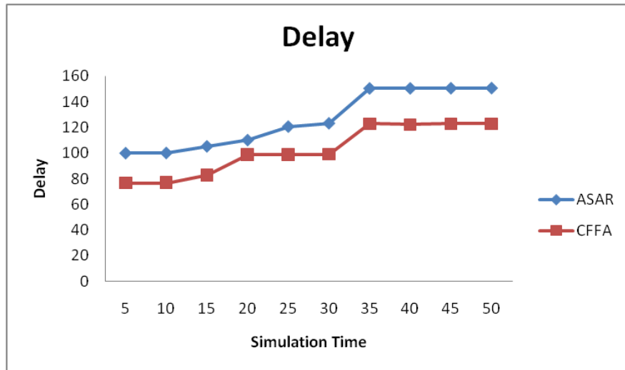
Figure. 3 Delay versus simulation time for ASAR and CFFA
