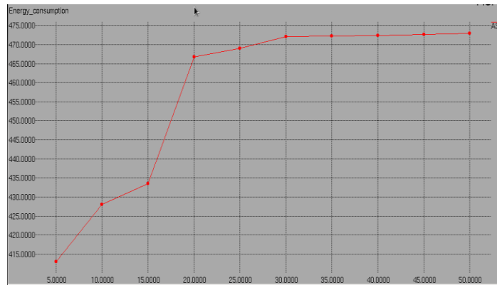
Figure. 4 To show the energy consumption on different Simulation Time on ASAR protocol.
