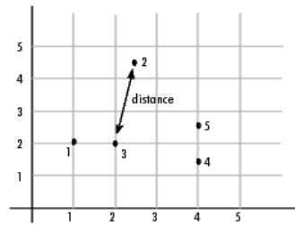
Fig 1-Hierarchical Clustering
