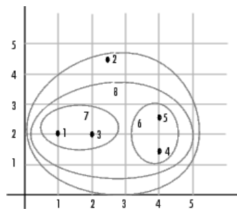
Fig 2-Linkage group using hierarchical Clustering
