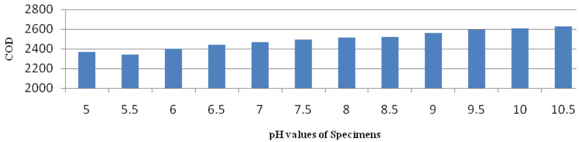
Graph 4: Variation in COD at different pH values for Lignin-water media after 90 minutes
