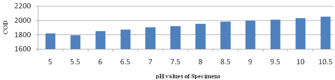
Graph 5: Variation in COD at different pH values for Lignin-water media after 120 minutes
