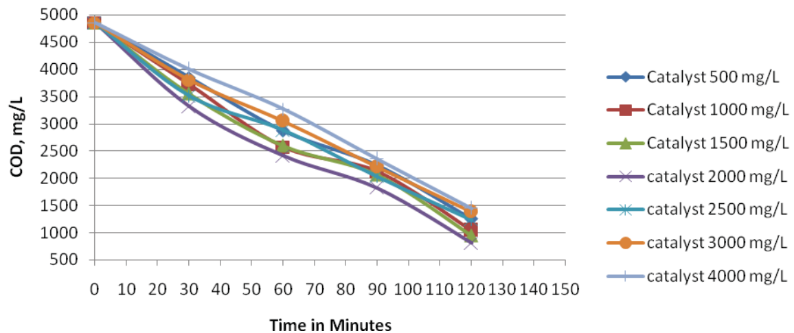
Graph 6: Variation in COD at different Catalyst Concentrations for Lignin-water media w.r.t. Time
