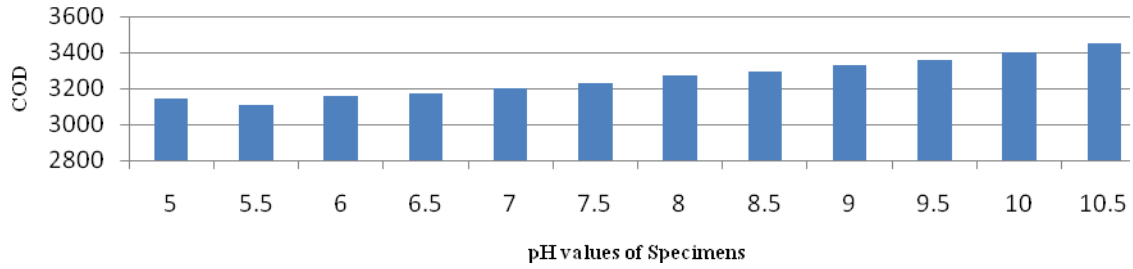
Graph 3: Variation in COD at different pH values for Lignin-water media after 60 minutes
