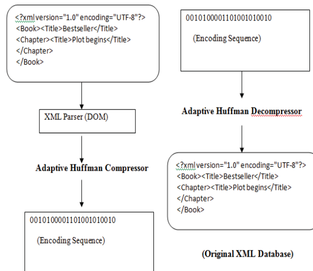
Fig: 1.2. XML Compression & Decompression Process
