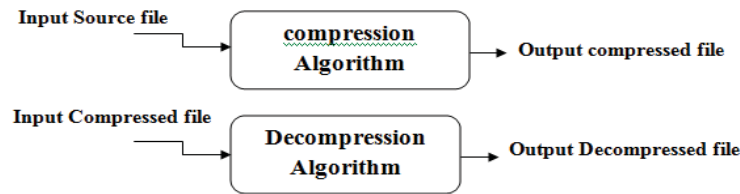
Fig 1.1: compression & Decompression
